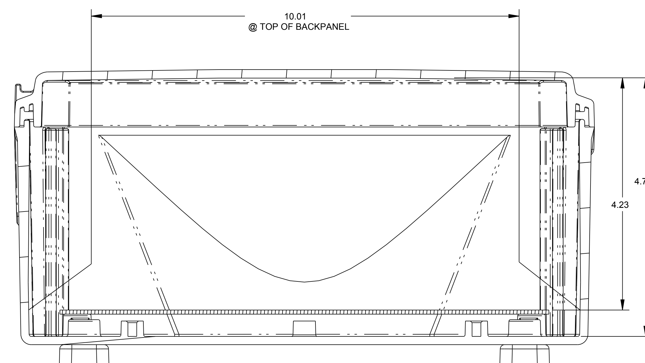
SECTION B-B
